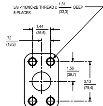
DETAIL "A" SYSTEM PORTS A & B SAE: 1.50" DIA. 8000 PSI (38.1" (414 BARS)) 4-BOLT FLG. CONNECTION
