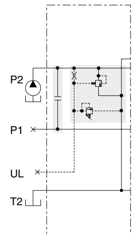
Standard inlet I with L-function and main pressure-relief function PS (P70CP, P70LS).
