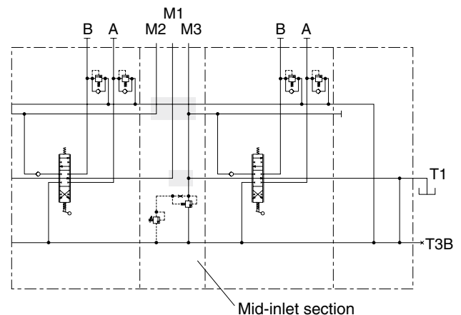
Mid-inlet, C6. Used for separate feeding (port M2) of non-prioritised sections upstream of the mid-inlet. See page 22.
